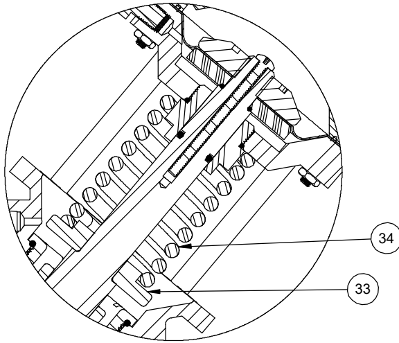
1071438 (K554-X203-14000) FAILSAFE SPRING CLOSED 100 PSI
