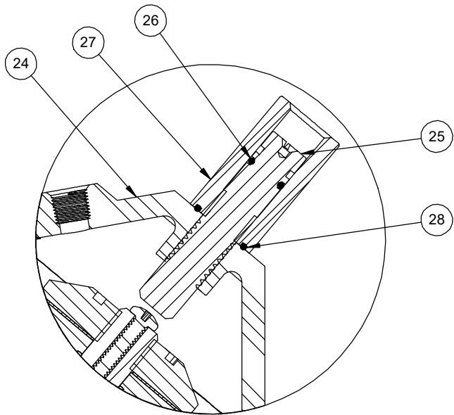
1079768 (K554-X210-14000) LIMIT STOP
