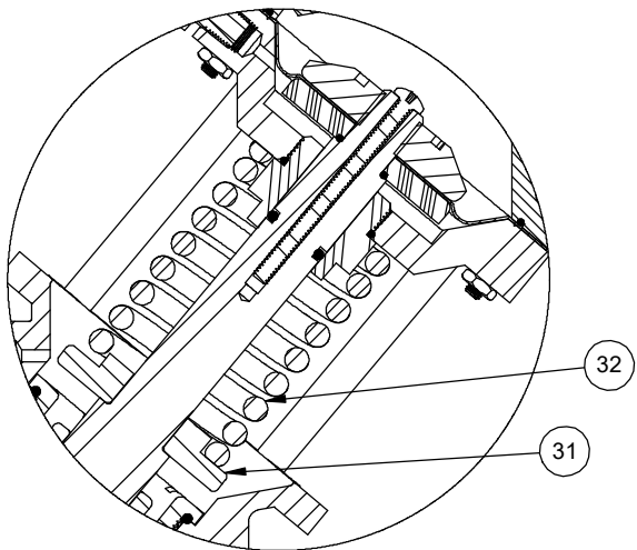
1071438 (K554-X203-14000) FAILSAFE SPRING CLOSED 60 PSI
